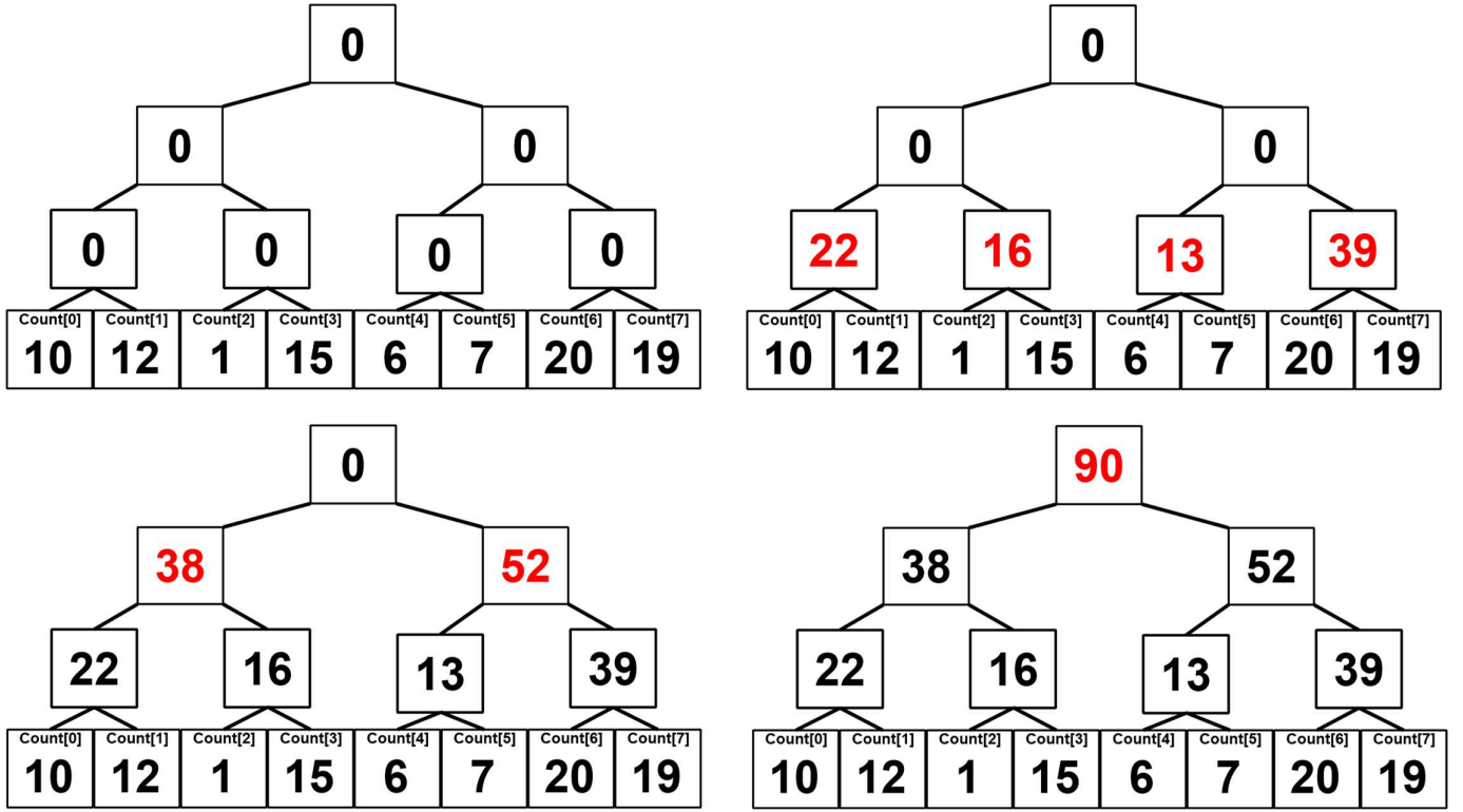
Figure 9: Bletloch scan up-sweep tree visualization.
