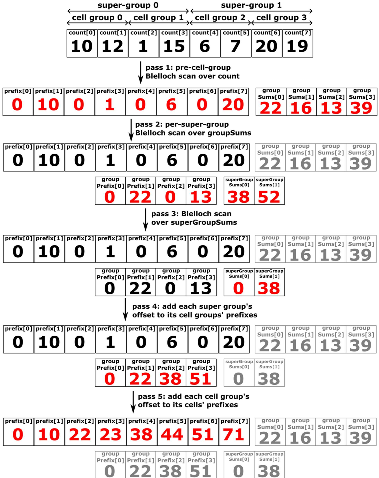
Figure 13: 5-pass hierarchical Blelloch scan.
