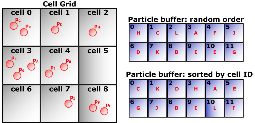
Figure 6: Unsorted vs sorted particle data in memory.
