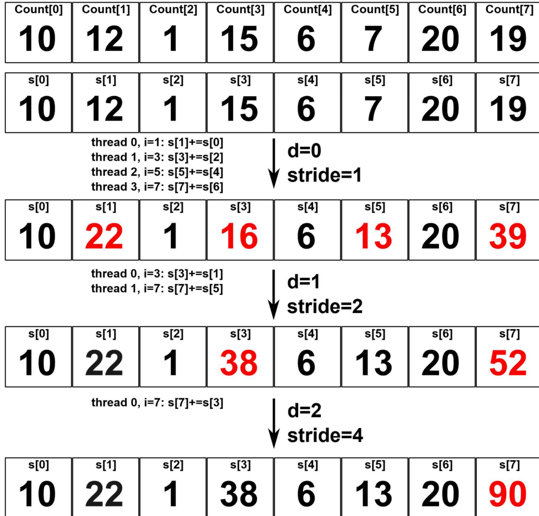
Figure 8: Bletloch scan up-sweep array visualization.
