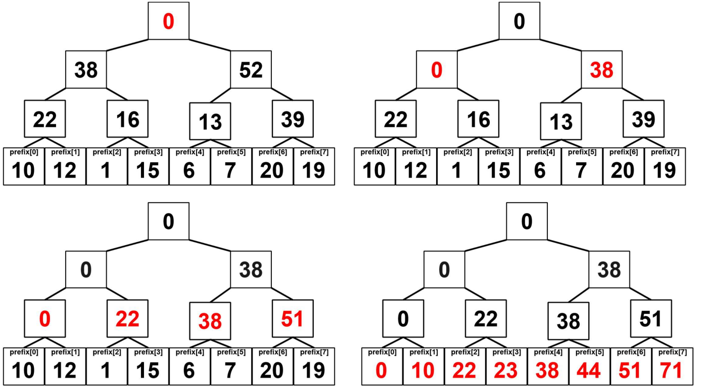
Figure 12: Bletloch scan down-sweep tree visualization.
