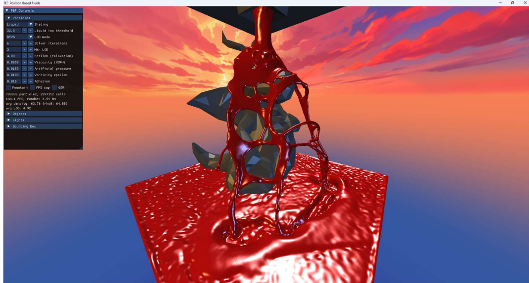
Figure 21: Liquid shading.
