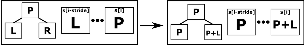
Figure 10: Bluelock scan butterfly.
