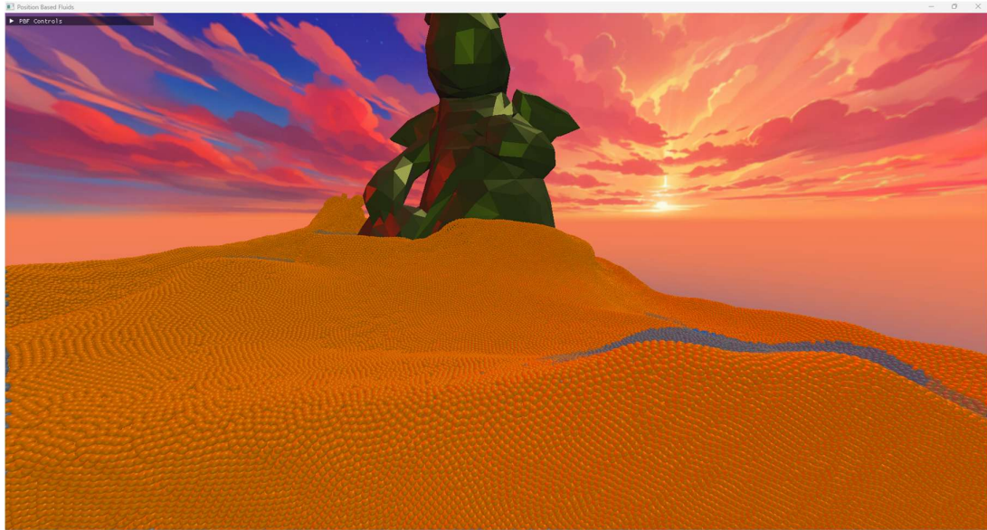
Figure 16: display for 2-frame LOD delay. Notice the rim of particles that got assigned a lower-than-expected LOD at the edge of the wave.
