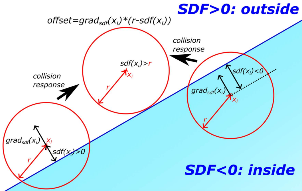
Figure 14: SDF collision detection and response.
