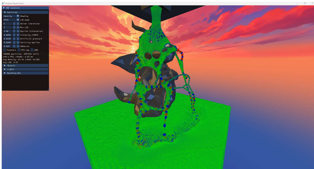
Figure 19: Density shading.
