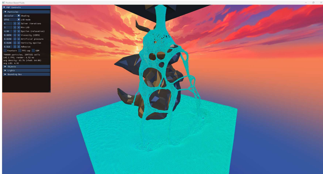
Figure 18: Unicolor shading.
