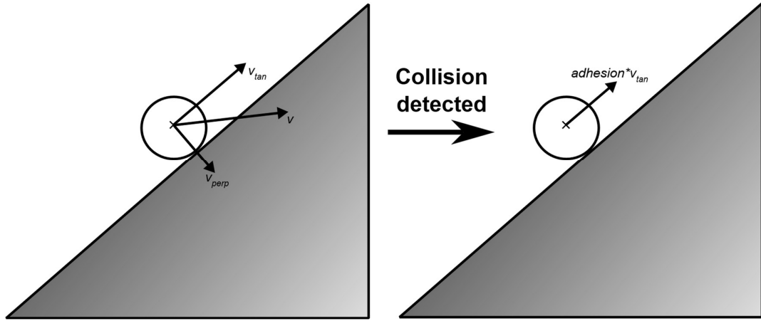
Figure 3: Collision velocity response.
