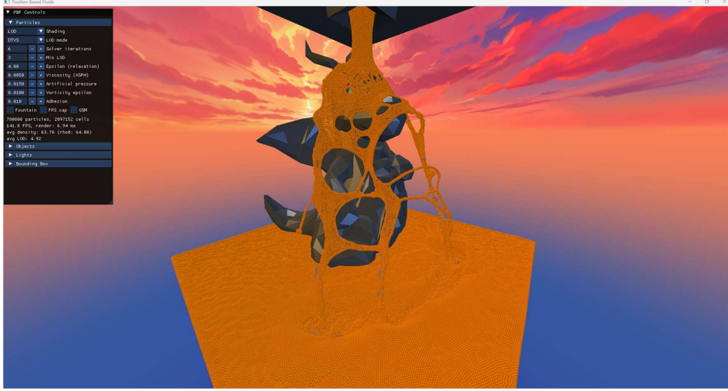
Figure 20: LOD shading.
