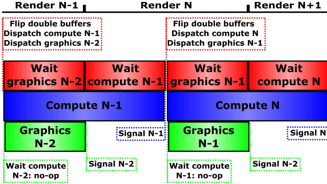
Figure 1: Compute-Graphics timeline.
